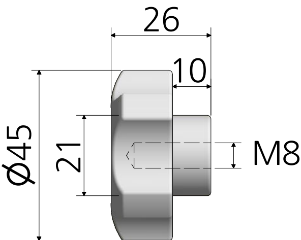
FKN-M8
