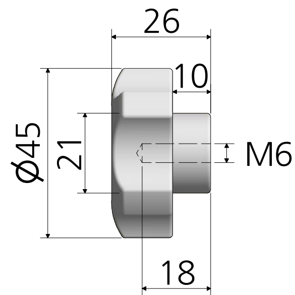
FKN-M6
